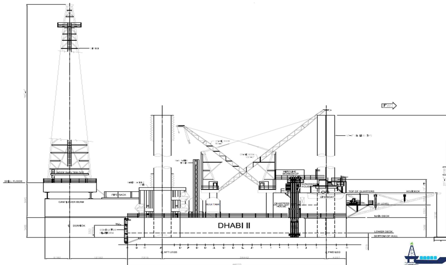
OUTER PROFILE
